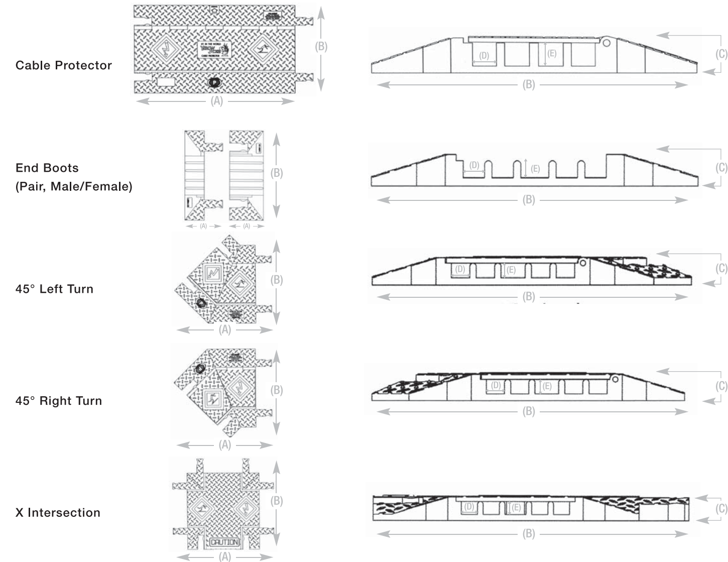
YJ5-125 cable protectors and accessories used as exemplary representations. Drawings are representational and are not necessarily to scale.
