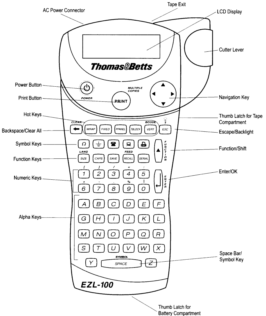
Figure 1 Thomas & Betts EZL-100 Thermal Label Printer
